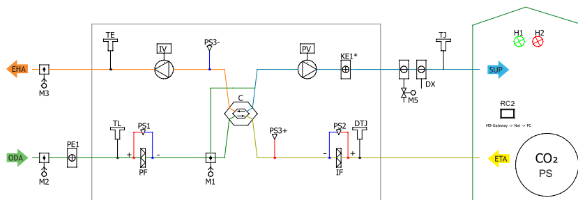
Рис. 15.2. RIS PW EKO 3.0 (* Placement of the component depends on model; PE1 - self-regulating preheater)
